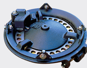
Precision mechanism with plates for seeds specifically drilled for each crop and grain sizes. Seed plates supplied per row: 01 for maize, 01 for soybeans and 01 blind plate.
