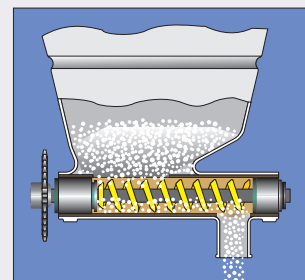
Auger type covered with PVC for precision and uniformity over the whole field.
